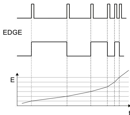
Figure 3-15 Types of count signal
