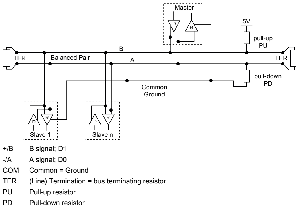
Figure 6-23 Block diagram: General topology of the twisted-pair cable
