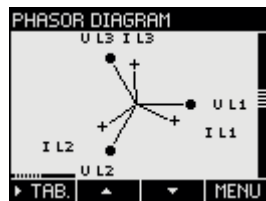
Figure 8-14 Phasor diagram
