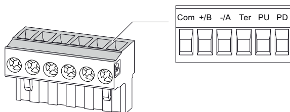
Figure 6-24 Terminal assignment
