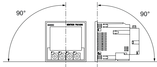
Figure 4-1 Mounting position
